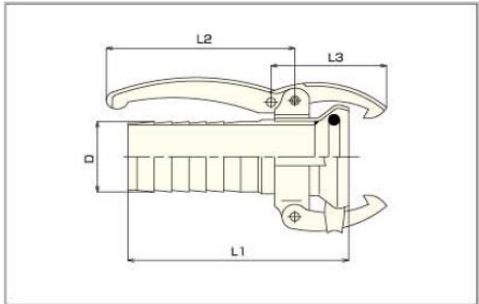
MN Hose Connect Type Sleeve (Female)
