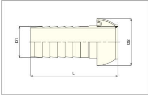
VN Hose Connect Type Sleeve (Male)
