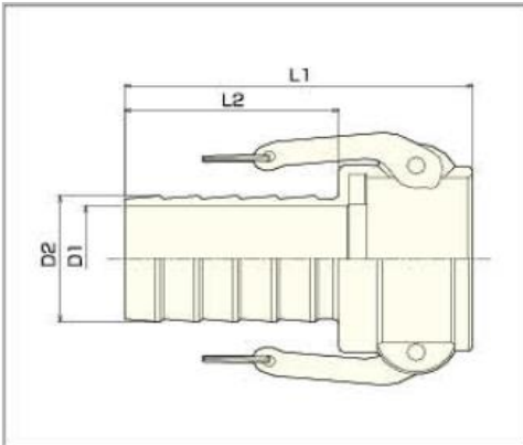
Structure (Cross-Section View)
