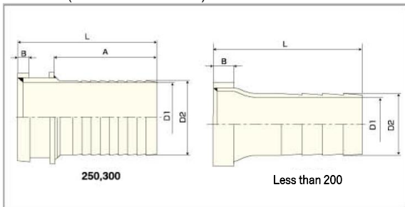
Structure (Cross-Section View)
